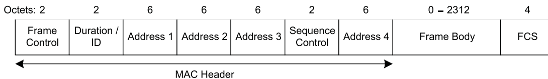
Figure 22—Data frame
