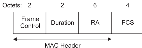
Figure 18—ACK frame
