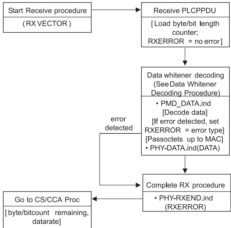
Figure 79—Receive state machine
