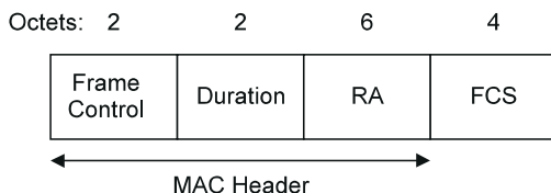
Figure 17—CTS frame
