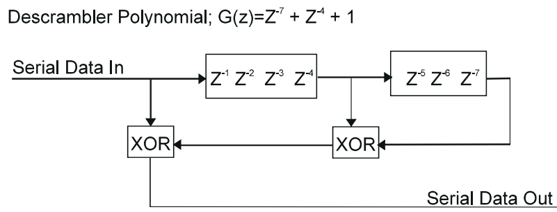
Figure 90—Data descrambler
