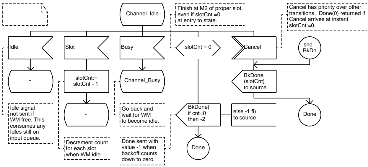
Process Backoff_Procedure
