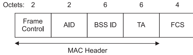
Figure 19—PS-Poll frame
