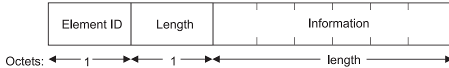
Figure 34—Element format
