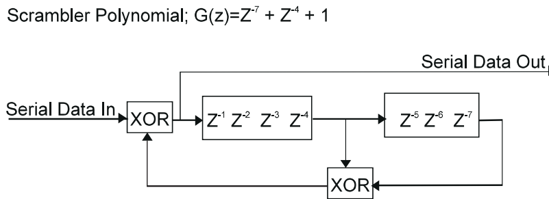
Figure 89—Data scrambler
