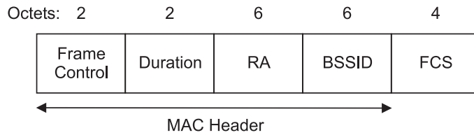
Figure 20—CF-End frame
