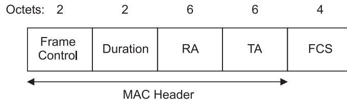
Figure 16—RTS frame
